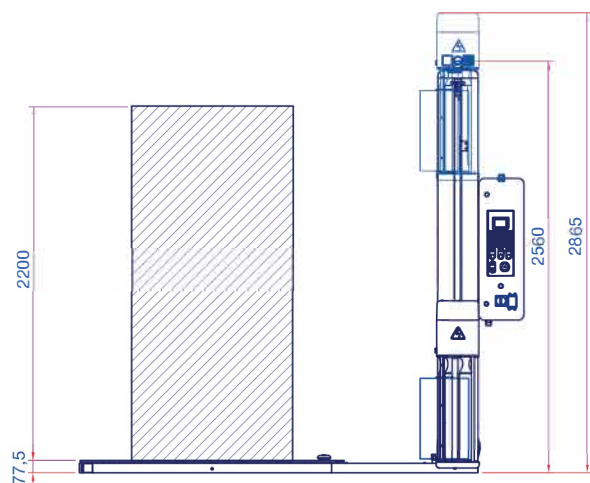
LAYOUT MASTERPLAT PLUS PGS [mm]
